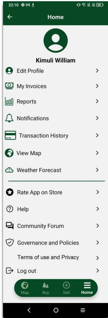
Home Screen
